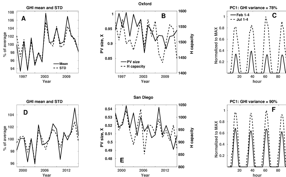
Figure 7: Panels A,D display GHI ( \text{kW}/\text{m}^2 ) over the entire interval. Panels B,E show PV size and H capacity during 18 model runs per geolocation using PV “pseudo-generation” as input, obtained from the 18-year GHI records as described in the main text. Required storage’s and PV’s size variability from year to year is portrayed. In Panels C,F the first principal component (PC1) of the 18 yearly timeseries is plotted for a few Winter and Summer days. PC1 accounts for the day-night cycle (crests and troughs with 24 hr period) and for the seasonal cycle (greater magnitude of Summer/dashed curves’ peaks with respect to solid curves’ peaks). PC1 is associated to 78% of variance in Oxford and to 90% of variance in San Diego; each higher order PCs explains less than 2% of variance in Oxford (less than 1% in San Diego). The significantly higher PC1’s variance in Southern California can be attributed to more stable weather with respect to the British Isles. Legend in Panel A refers also to Panel D ; the same holds for Panels B and E and for C and F .
