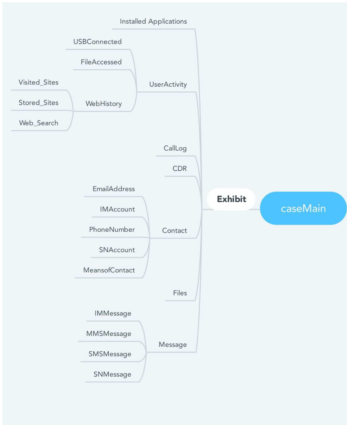
Figure 12. Ontology Class Hierarchy
