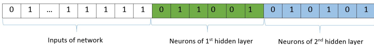
Figure 2: A chromosome representing a network architecture
