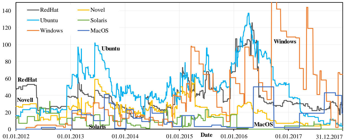
Fig. 4. Forever-day vulnerabilities.
