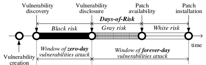
Fig. 1. Vulnerability lifecycle.
