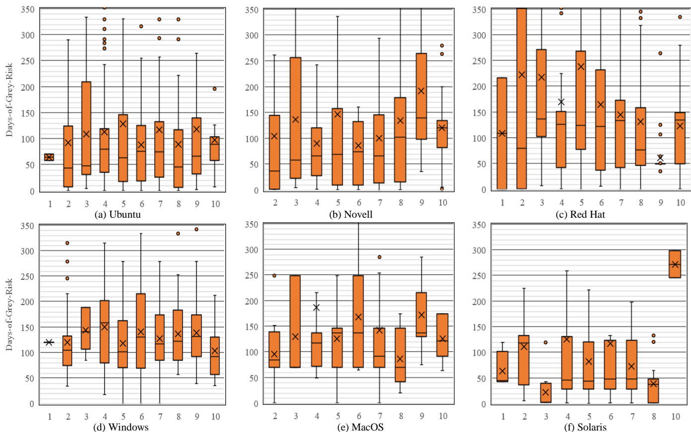
Fig. 7. Box-and-whisker diagrams showing a days-of-gray-risk statistics (Y-axes) for vulnerabilities of different CVSS severity scores (X-axes)
