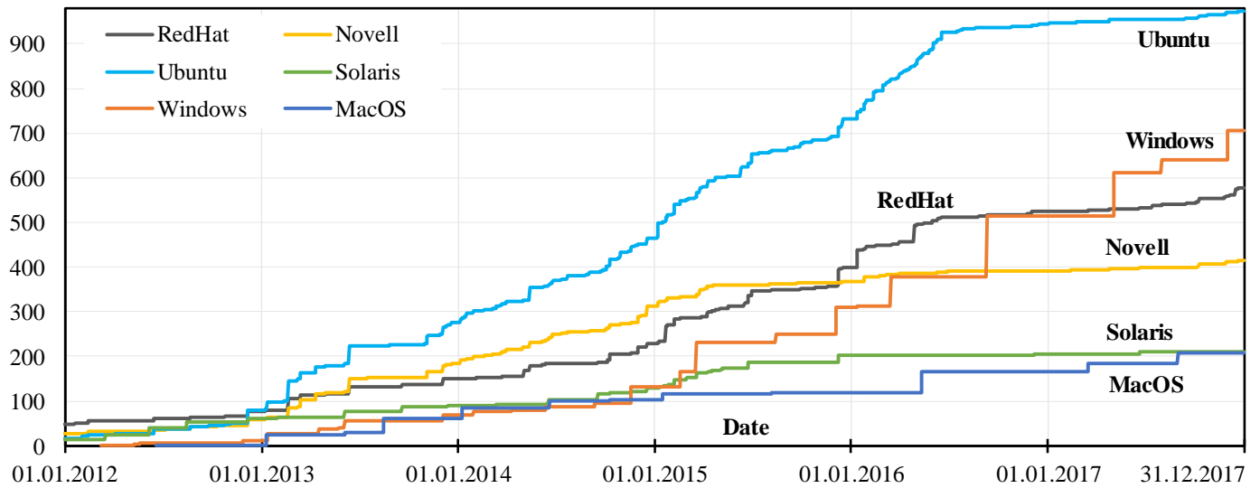
Fig. 3. Cumulative number of disclosed vulnerabilities.
