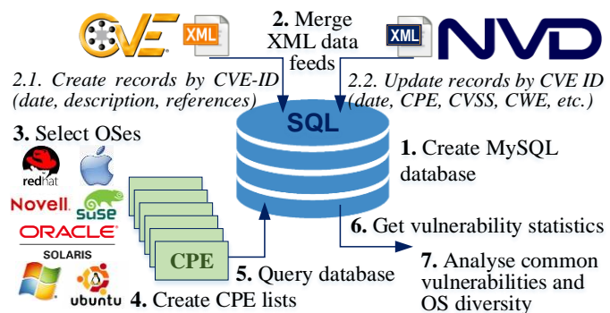
Fig. 2. Research methodology.
