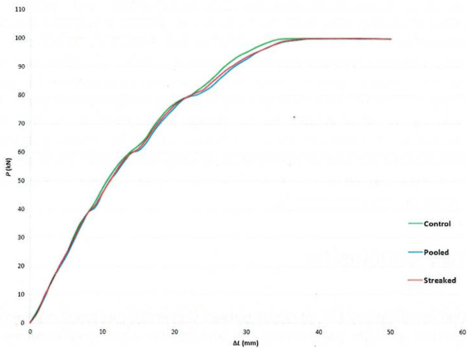
Figure 3-2 Averaged plot of P \ v \ \Delta L for all control, pooled and streaked samples.
