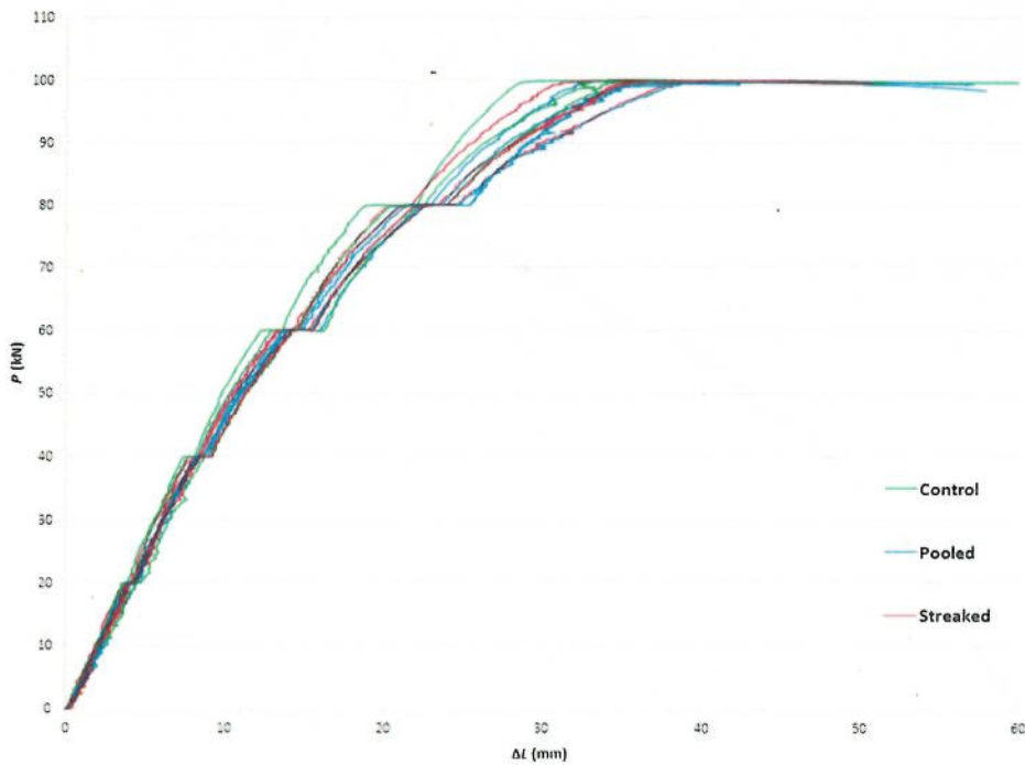
Figure 3-2 Data plot of P \ v \ \Delta L for all control, pooled and streaked samples.
