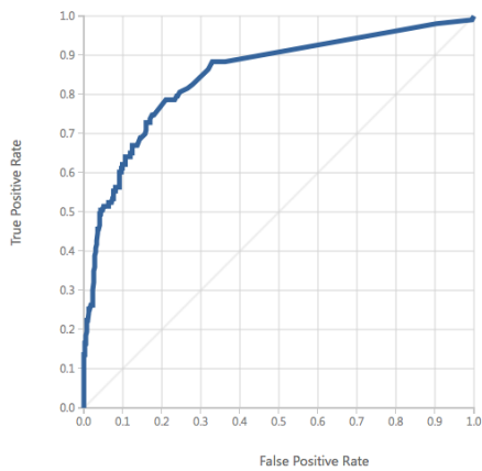
Figure 10 : The ROC curve for model 2
