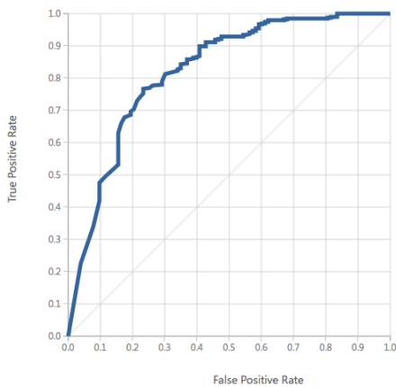
Figure 8 : The ROC curve for model 1
