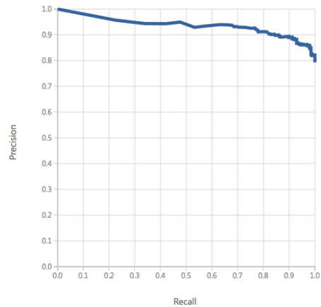
Figure 9 : The Precision-Recall curve for model 1
