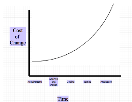
Figure 3: Ambler’s traditional cost of change curve
