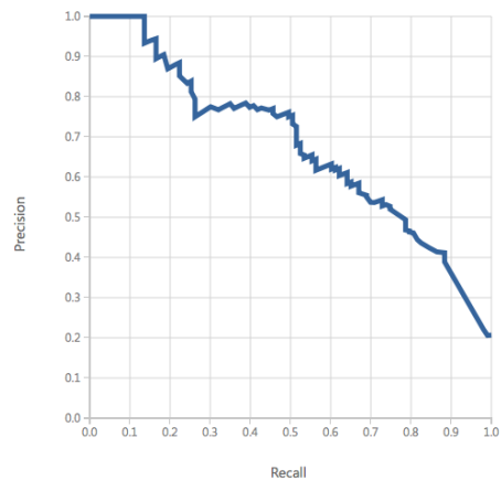
Figure 11 : The Precision-Recall curve for model 2
