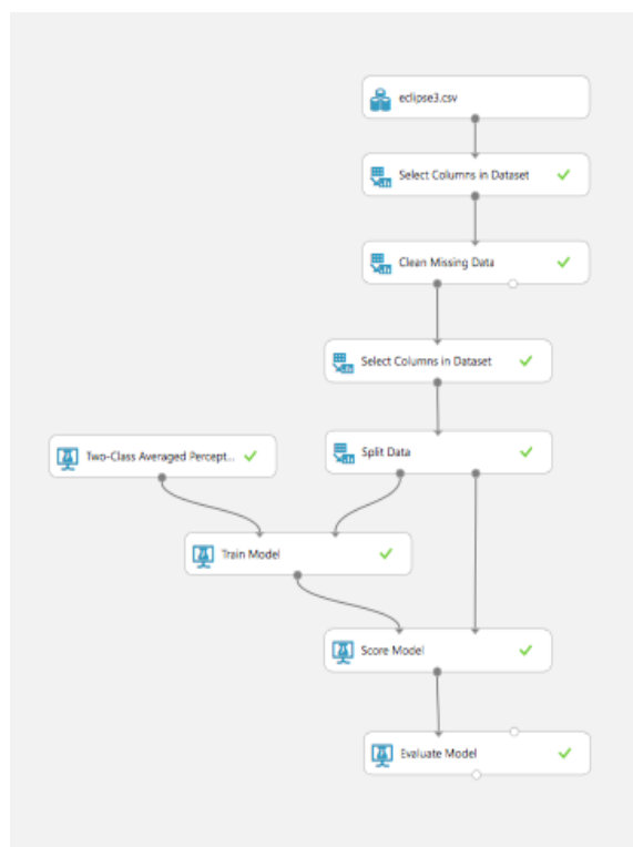
Figure 6: Schematic flowchart of the machine learning experiment in Azure.
