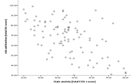
Figure 5.1e. ASD: Scatterplot showing state anxiety correlated with job satisfaction ( r_s = -.51, p < .001 )
