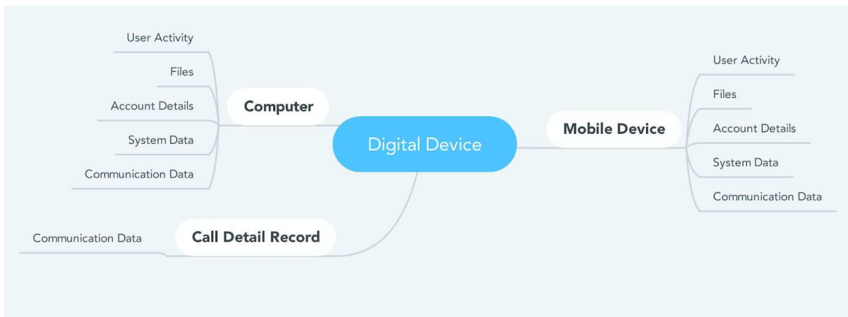
Figure 2. Digital Hosts
