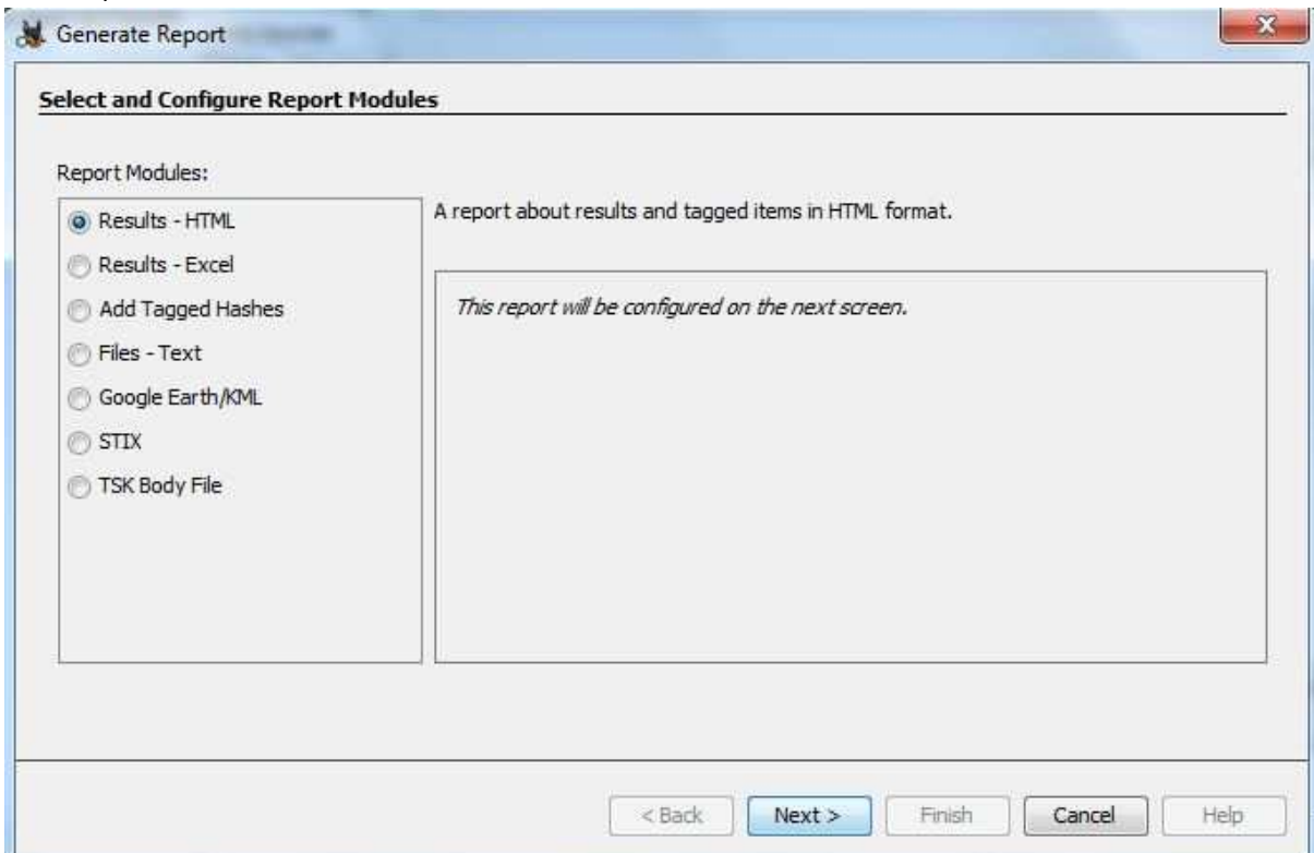
Figure 5. Autopsy Outputs
