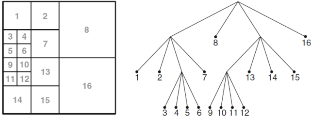
FIGURE 4. An example of HEVC's 64X64 luma CTU partitioned into CUs of 8x8 to 32X32 luma samples, with the numbers representing the coding order of the CUs [7]
