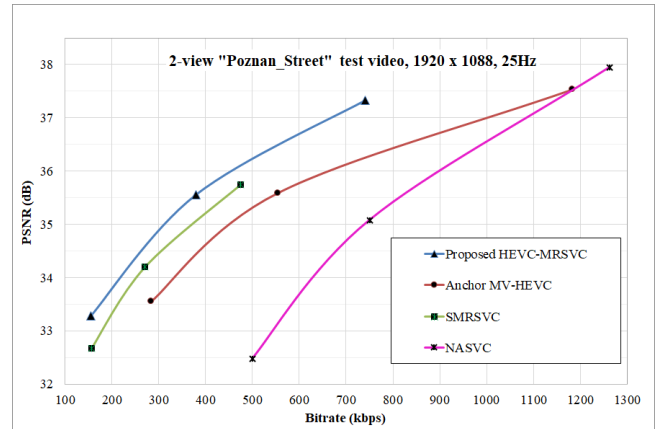
FIGURE 15. PSNR versus bitrate for coding “Poznan_street” stereo videos using proposed HEVC-MRSVC, anchor MV-HEVC, SMRSVC and NASVC codecs.
