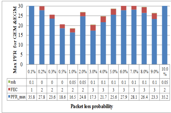
Figure 2. Maximum PFR vs the probability of packet loss and packet correlation.
