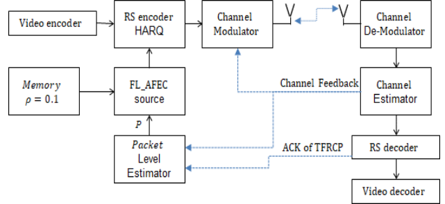
Figure 3. FL_AFEC Processing Blocks.
