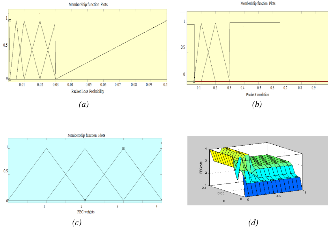
Figure 5. FL_AFEC: Mamdani Fuzzy –Logic Based on Triangular-Shape; (a) Membership of Linguistic Variable P; (b) Membership Linguistic Variable \rho ; (c) Membership of Output FEC; and (d) Fuzzy Logic System Decision Surface.
