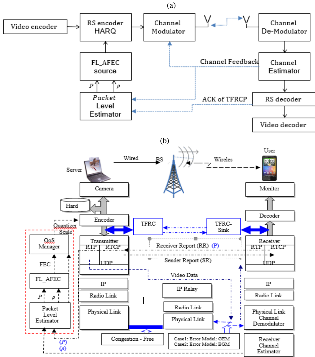
Figure 1. (a) System process; (b) video streaming architecture in which Fuzzy logic is considered to control the FEC.
