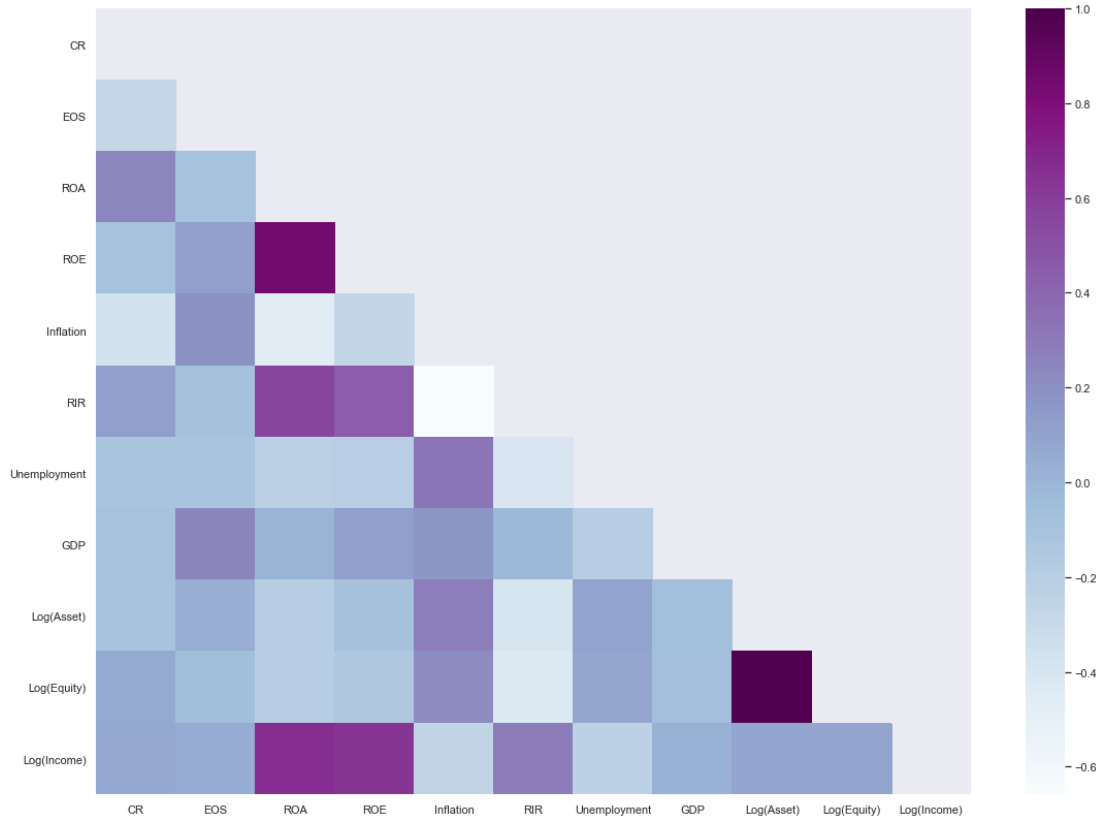
Figure 1. Correlation matrix
