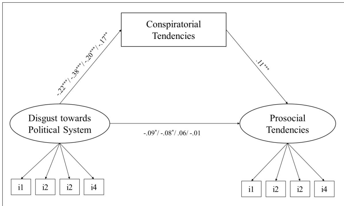
Figure 1. Structural equation model showing unstandardized coefficients.
