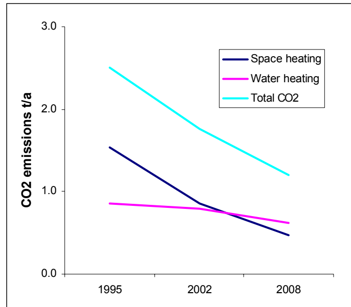
Figure 3.7 Comparisons of carbon emissions under ADL95, ADL02 and EPS08, for an 80 m² gas heated semi-detached dwelling.
