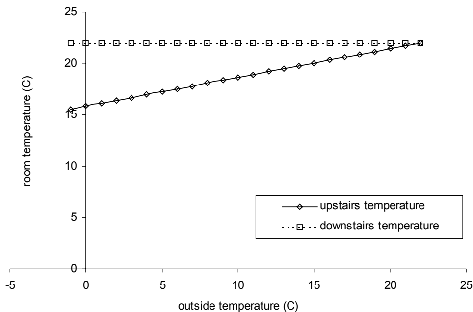
Figure (1). Temperature drop in unheated upstairs rooms.
