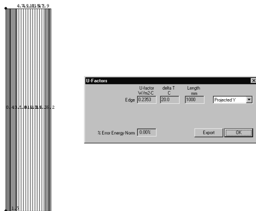
Figure (3): U factor of wall = 0.2353 W/m²K
