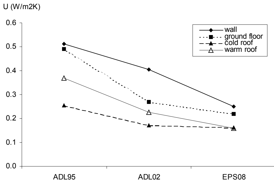
Figure 4.11: Elemental U values including linear thermal bridging.
