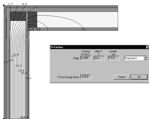
Figure (4): Isolines at junction using adiabatic conditions on the RHS wall. U factor of junction = 0.2985 W/m²K
