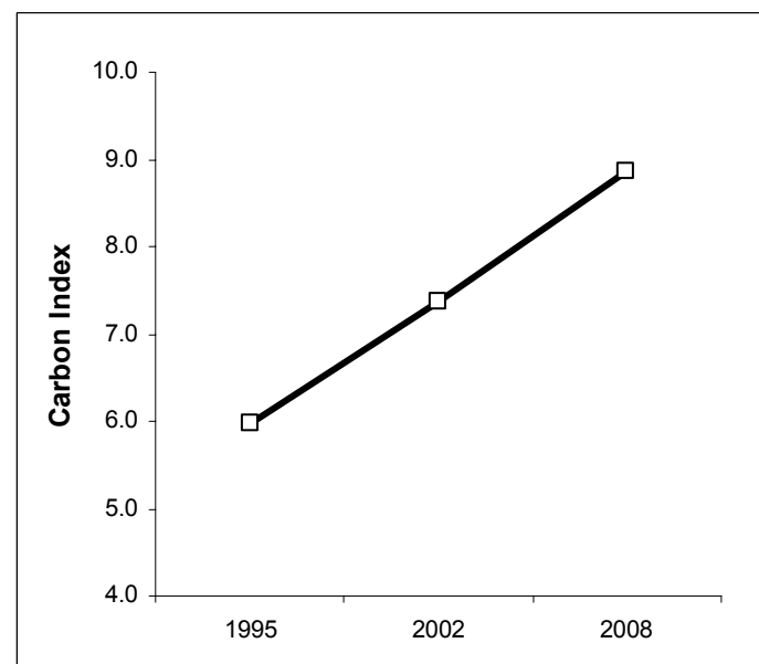
Figure 3.8 Comparisons of carbon index under ADL95, ADL02 and EPS08, for an 80 m² gas heated semi-detached dwelling.
