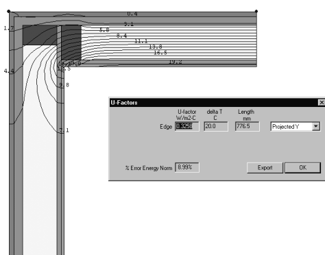
Figure (5): Isolines at junction using adiabatic conditions on the LHS wall. U factor of junction = 0.3258 W/m²K.
