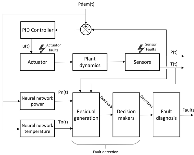
FIGURE 2. Block diagram of the fault detection approach.
