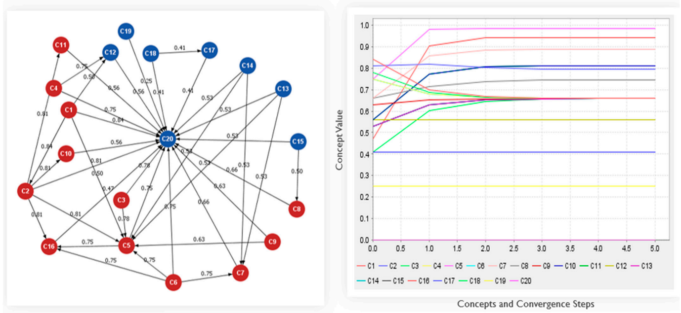
Figure 4. Initial mapping test output with associated convergence output plot: the x-axis shows the steps to convergence for a particular iteration; the y-axis shows the converged value of concepts contributing to the startle output.
