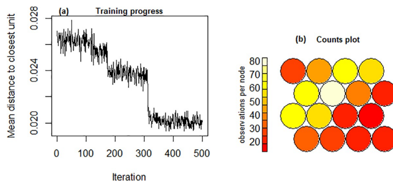
Fig 4. (a). SOM convergence during the training. (b). Count plot representing the records per node in SOM map for pMan-HD data.
