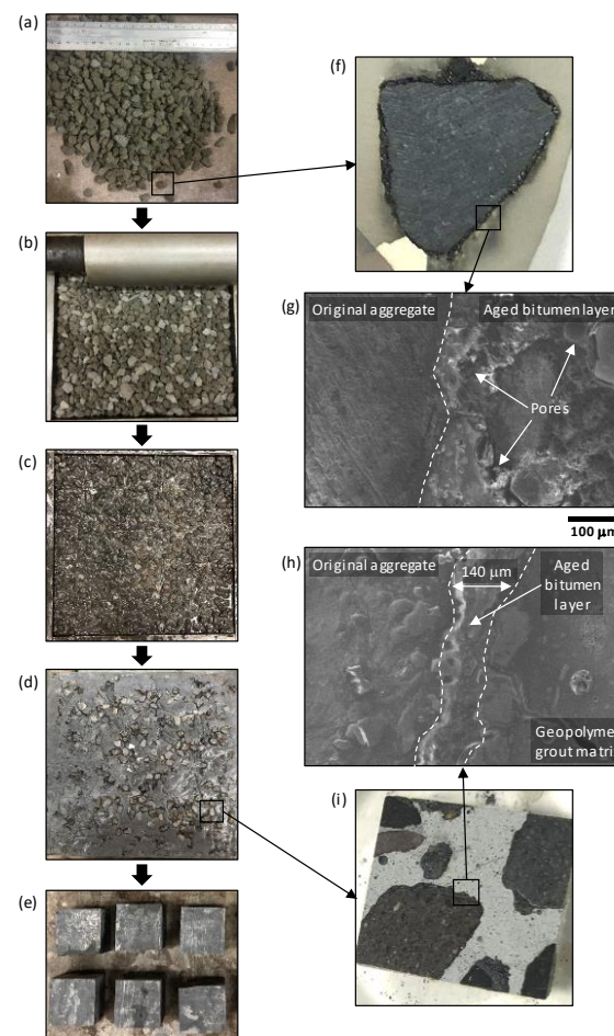
Figure 1. SFC manufacturing steps, including: (a) preparation of single-sized RAP particles; (b) hand compaction of RAP particles; (c) RAP particles infused with fresh geopolymer grout; (d) hardened SFC slab (200 × 200 × 50 mm); (e) extraction of SFC specimens for testing (50 mm cubes for compressive strength testing shown); (f,g) SEM characterisation of RAP particle; and (h,i) SFC specimen.
