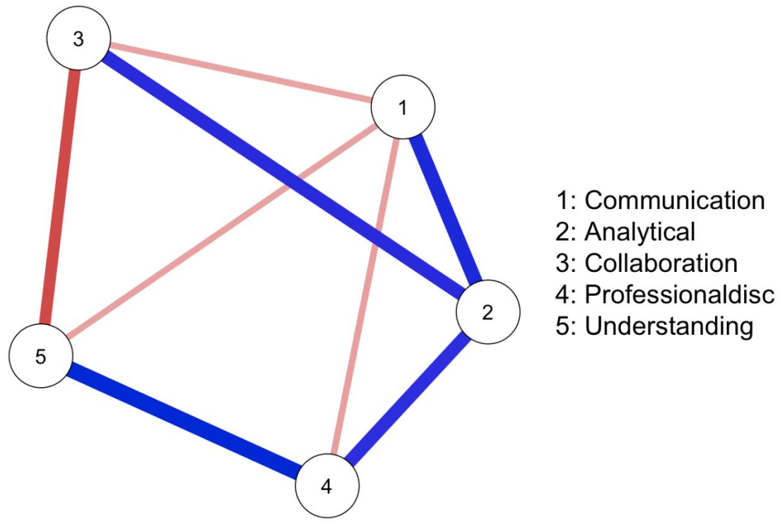
Figure 4: HNC network plot
