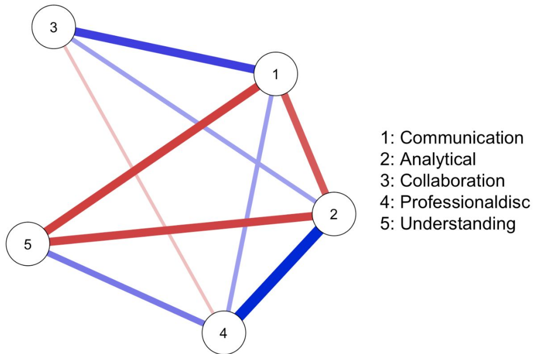
Figure 5: HND Network plot
