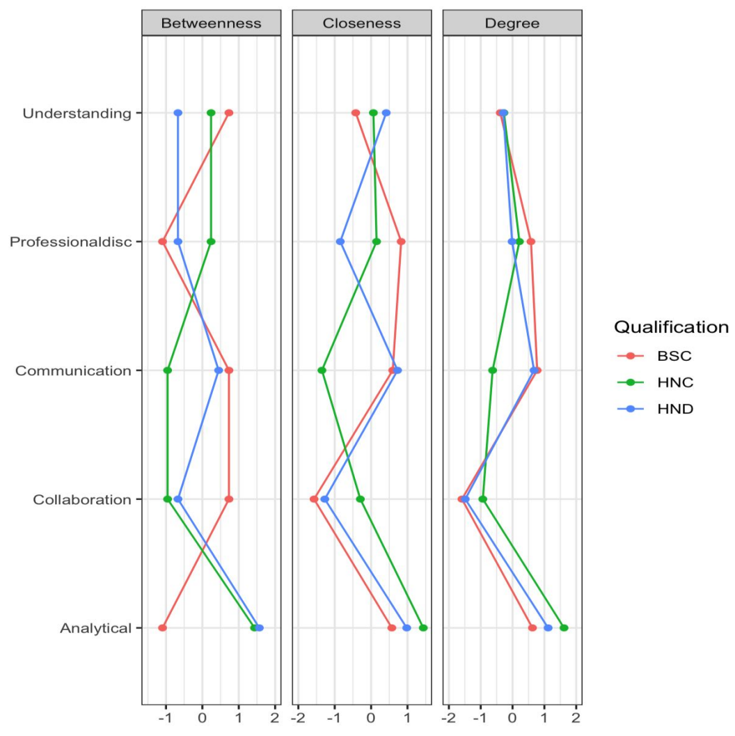
Figure 6: Centrality plot for BIM pedagogy
