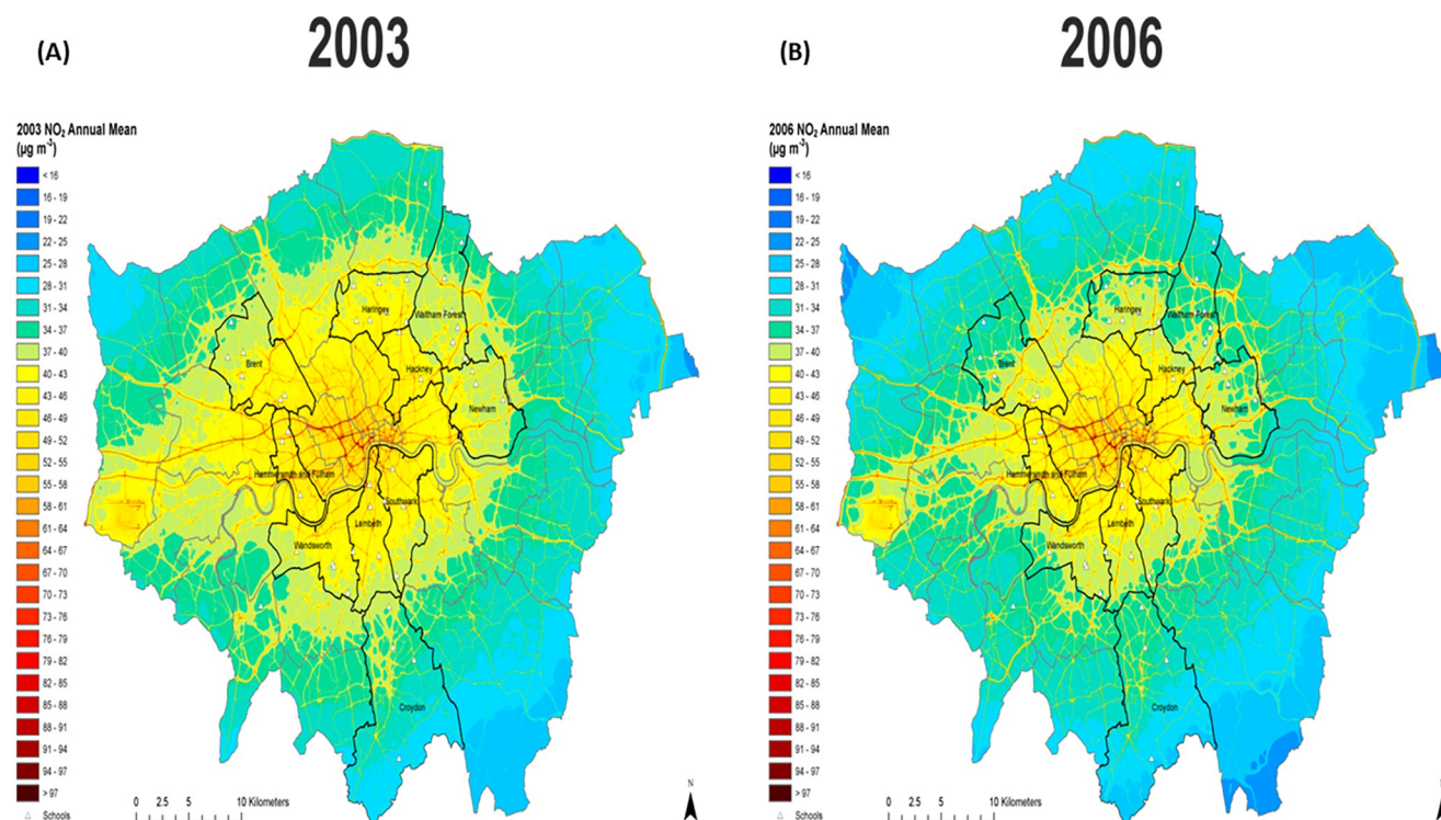
Fig 2. Modelled Greater London concentrations (20m 2 resolution) for NO 2 for representative years 2003 (A) and 2006 (B). The ten boroughs in which the study took place are highlighted together with the locations of the participating schools (open triangles).
