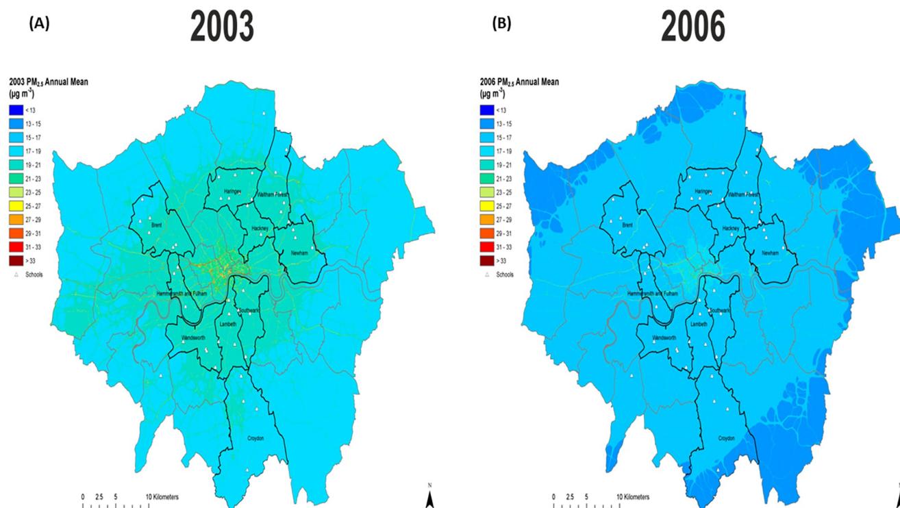
Fig 1. Modelled Greater London concentrations (20m 2 resolution) for PM 2.5 for representative years 2003 (A) and 2006 (B). The ten boroughs in which the study took place are highlighted together with the locations of the participating schools (open triangles).
