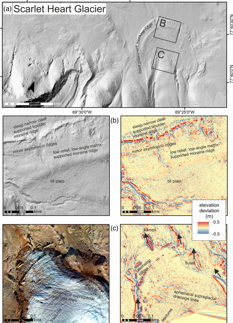
FIGURE 6 (a) Microtopography, geomorphology, land surface texture, and glacier surface structure at Scarlet Heart Glacier. We highlight parts of the contemporary ice margin (b) and the proglacial area (c) using a mosaic high-resolution (0.02 m) orthophotograph, a hillshaded image of a high-resolution (0.2-m XY grid) digital elevation model, and as elevation deviations from a 10-m spatial mean. Arrows in (c) denote major abandoned water pathways. The full extent of these datasets is depicted in Supporting Information S1.
