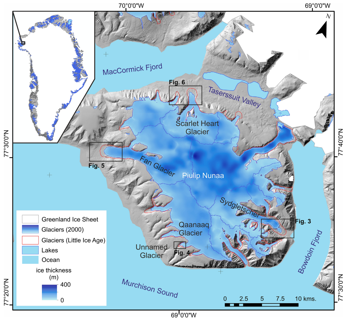
FIGURE 1 Location of Qaanaaq ice cap and names of outlet glaciers focussed on in this study. Glaciers (year 2000 from the RGI_v6.0) are from GLIMS (Raup et al., 2007), ice thickness is from Millan et al. (2022), and the background is a hillshaded image of the ArcticDEM mosaic (Porter et al., 2018).
